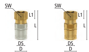
Couplings with straight female thread without/with valve
