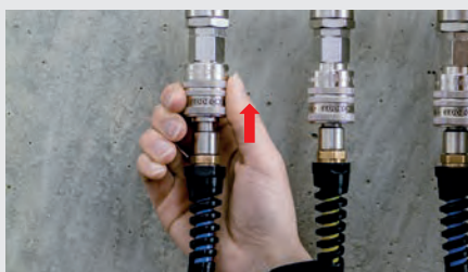
Disconnection - first step: Automatic venting
