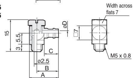
M-5ALHN-6 M-5ALHU-6
